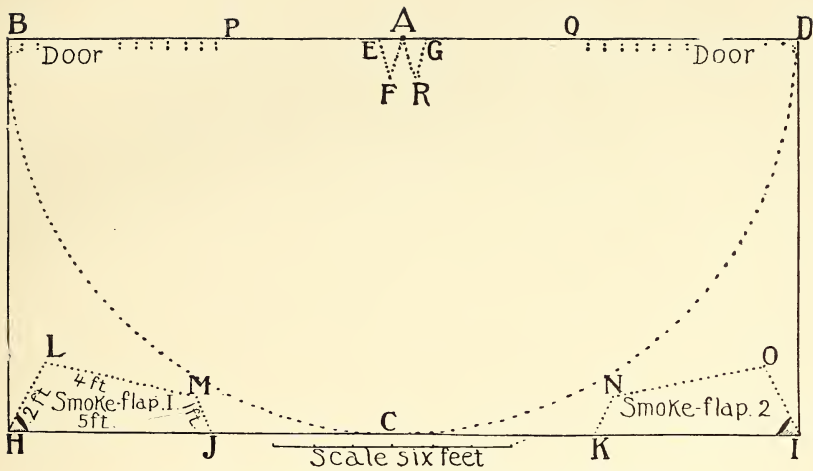
CUT I.—PATTERN FOR A SIMPLE 10-FOOT TEEPEE
